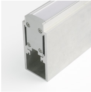
KKFR-03* Ground box Anodised aluminium finish W37.6/H80.9mm (W1.48/H3.19") * Specify length to match MOMO-F
